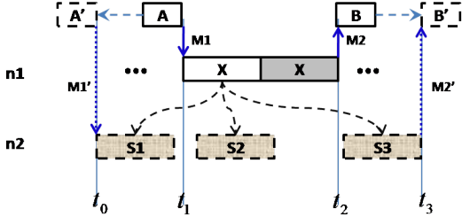
Figure 7: Influence of Data Dependency on Task Migration
