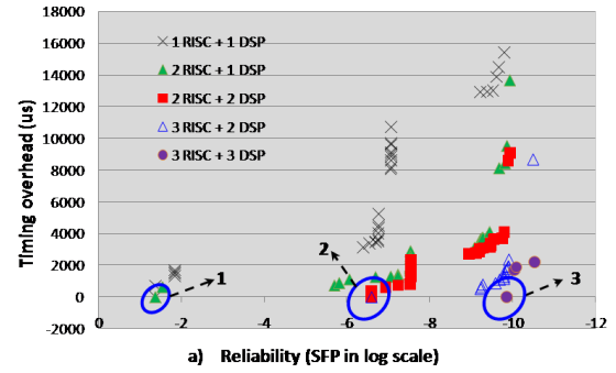
Figure 9: Pareto Optimal Solutions under Different Platform Configurations
