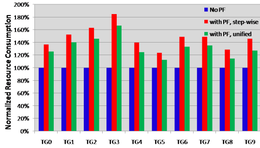
Figure 11: Performance Comparison of Step-wise and Unified Approaches
