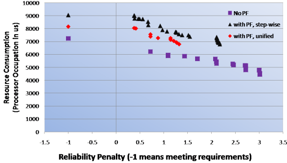
Figure 11: Performance Comparison of Step-wise and Unified Approaches
