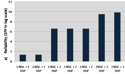
Figure 9: Pareto Optimal Solutions under Different Platform Configurations
