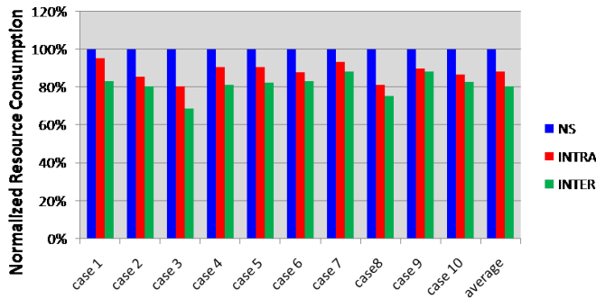
Figure 13: Comparison of Slack Sharing Schemes
