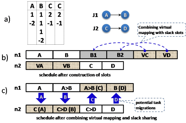
Figure 8: Example of Virtual Mapping
