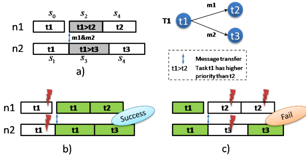
Figure 2: Example Fault Scenario
