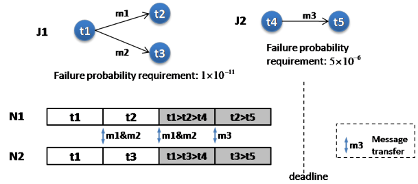
Figure 4: Example of Static Priority Slack Sharing
