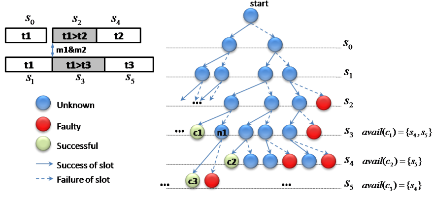
Figure 3: An Example of Binary Tree Analysis
