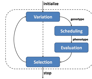
Figure 5: Workflow of EA-based Optimization
