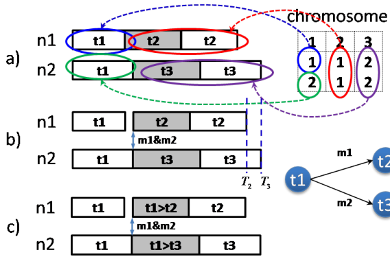
Figure 6: Encoding and Reconstruction of Schedule
